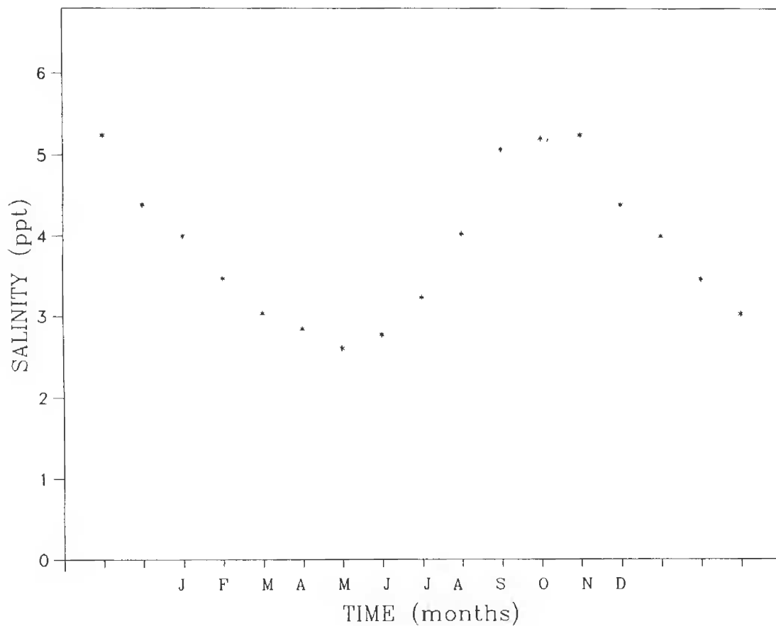
Figure 2. Monthly mean salinity.
